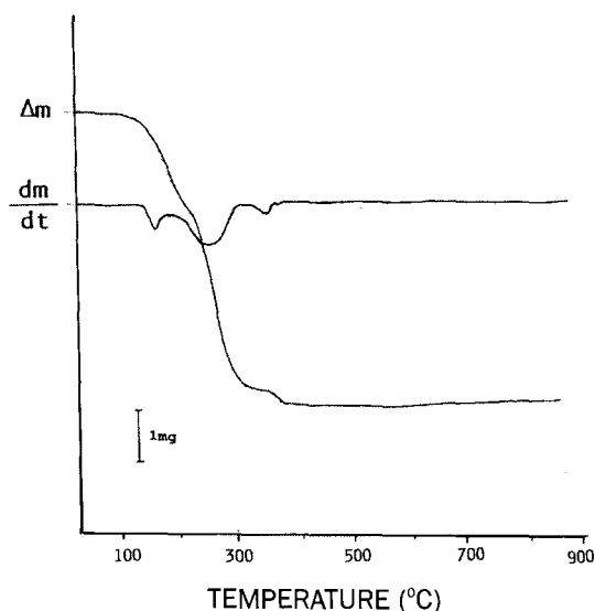
Figure 1. Simultaneous TG/dTG curves of [\text{Pd}_2(\text{dmba})_2(\mu\text{-SO}_4)(\text{SO}_2)_2] .
