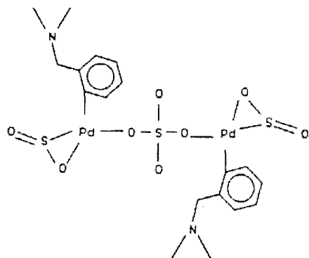
Figure 2. Schematic drawing of [\text{Pd}_2(\text{dmba})_2(\mu\text{-SO}_4)(\text{SO}_2)_2]
