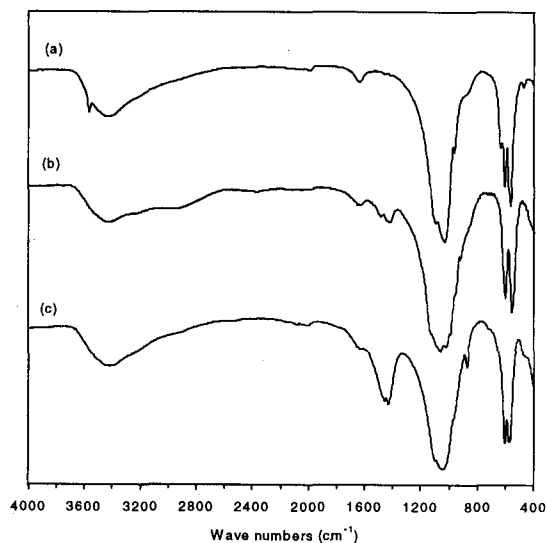
Figure 2. FTIR spectra of the material (a) commercial, (b) synthesised without the presence of NH 4 F and (c) in presence of NH 4 F.
