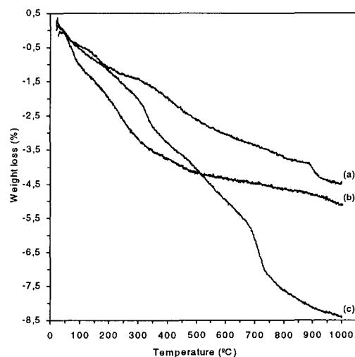
Figure 3. TG diagrams of the material (a) synthesised without the presence of NH 4 F, (b) commercial and (c) synthesised in the presence of NH 4 F.
