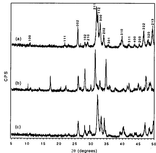
Figure 1. XRD patterns of the material (a) commercial, (b) synthesised without the presence of NH 4 F and (c) in presence of NH 4 F.
