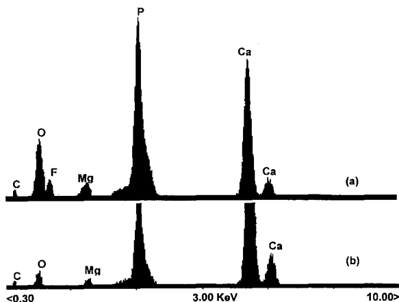
Figure 4. EDX patterns of the material (a) synthesized with \text{NH}_4\text{F} addition in the reaction and (b) in \text{NH}_4\text{F} absence. Accelerating voltage of 25keV.
