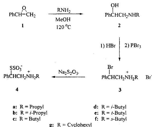
Scheme 1. Formation of 2-(alkylamino)-1-phenyl-1-thiosulfuric acids
