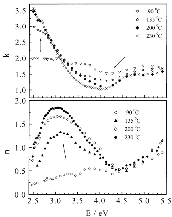
Figure 8. Optical parameters ( k and n ) measured for PTHT films converted into PPV films at different temperatures
