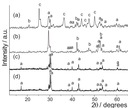
Figure 1. XRD patterns recorded for \text{Sr}_2\text{CeO}_4 prepared from (a) \text{SrCO}_3 and \text{CeO}_2 fired at 1000\text{ }^\circ\text{C} , 4 h; (b) polymeric precursor heated at 1100\text{ }^\circ\text{C} , 4 h 11 ; precursor from combustion method by using (c) citric acid or (d) glycine as fuels, heated at 950\text{ }^\circ\text{C} , 4 h. a = \text{Sr}_2\text{CeO}_4 8 , b = \text{SrCeO}_3 , PDF n. 83-1156 15 , c = \text{SrCO}_3 , PDF n.71-2393 15
