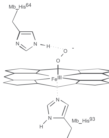
Figure 3. Electronic distribution and metal-ligand geometry of Fe-O 2 in oxymyoglobin illustrating the importance of His binding
