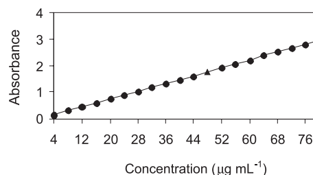
Figure 6. Beer's law verification range
