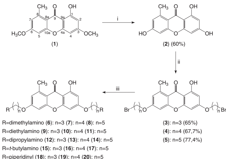
Scheme 1. Reagents and conditions: i) BBr_3 , CH_2Cl_2 , N_2 , rt, 16 h; ii) K_2CO_3 , acetone, Br(CH_2)_nBr , n=3, 4 or 5 , rt, 24 h; iii) amine (dimethyl, diethyl, dipropyl, t -butylamine and piperidine), acetone, rt, 48 h
