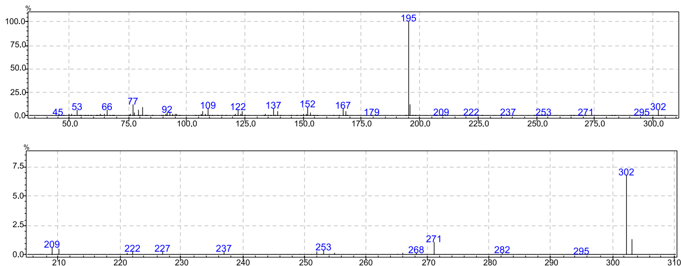
Figure 15S. EI-MS spectrum of 4c
