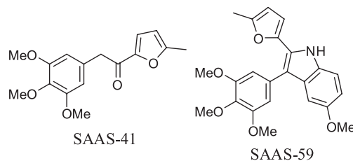
Figure 2. Structures of SAAS-41 e SAAS-59
