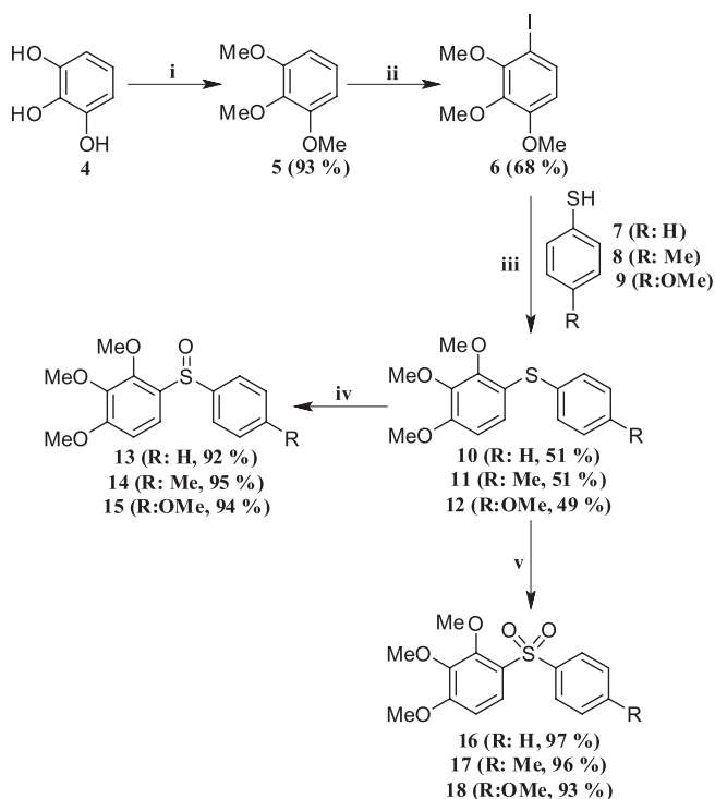
Scheme 1. Synthesis of CA-4 analogues. Reagents and conditions: (i) \text{CH}_3\text{I} , \text{K}_2\text{CO}_3 , acetone, \Delta ; (ii) NIS, TFA, acetonitrile, r.t.; (iii) neocuproine, CuI, t -NaOBu, toluene, 110 °C; (iv) 1 equiv. m -CPBA, \text{CH}_2\text{Cl}_2 ; (v) 2 equiv. m -CPBA, \text{CH}_2\text{Cl}_2
