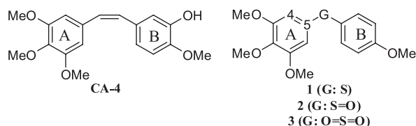
Figure 1. Structures of compounds 1, 2 and 3
